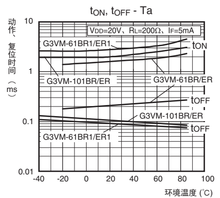
G3VM-61BR/61ER/61BR1/61ER1/101BR/101ER
