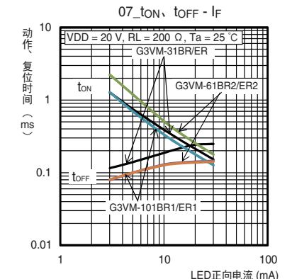
G3VM-31BR/31ER/61BR2/61ER2/101BR1/101ER1
