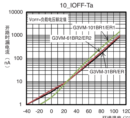
G3VM-31BR/31ER/61BR2/61ER2/ 101BR1/101ER1
