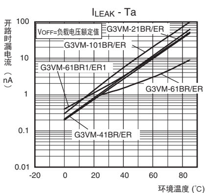
● 开路时漏电流—环境温度 G3VM-21BR/21ER/41BR/41ER/61BR/ 61ER/61BR1/61ER1/101BR/101ER
